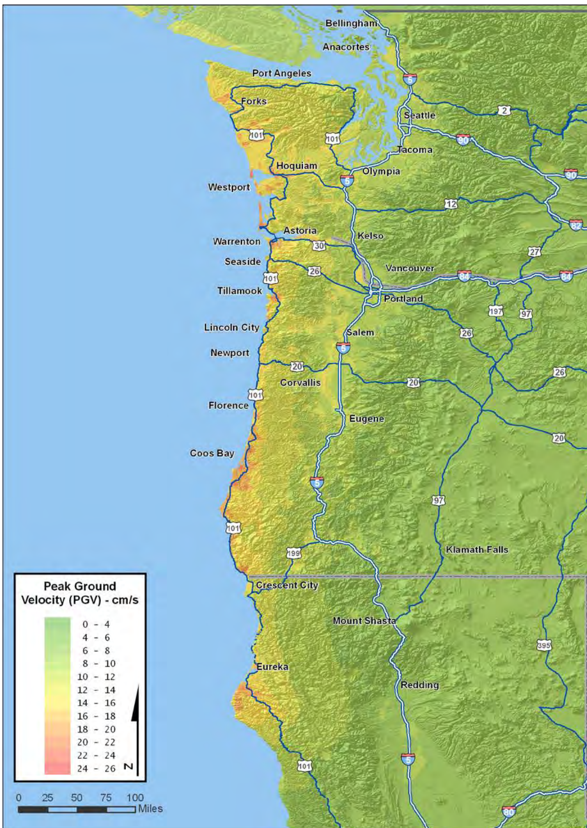
Figure 2-3. Peak ground velocity (cm/s)
