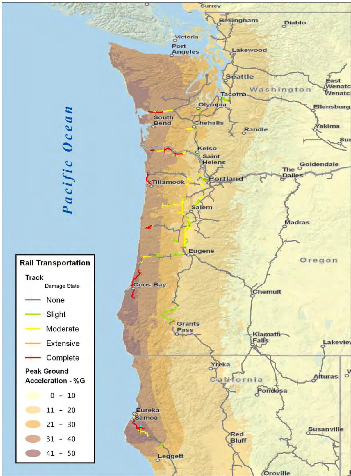
Figure 4-35. Damage to railroad track for the 50th-percentile (expected) case
