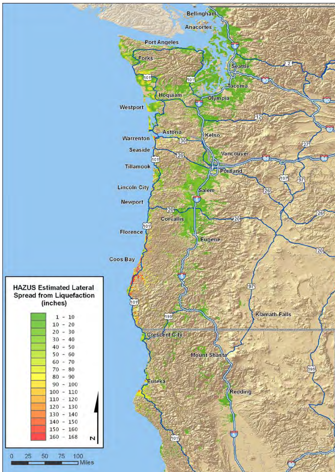
Figure 2-4. Hazus estimated lateral spread from liquefaction (inches)
