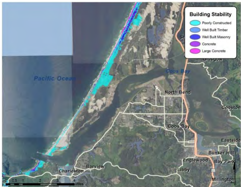
Figure B-33. Predicted building stability rating for Coos Bay, OR
