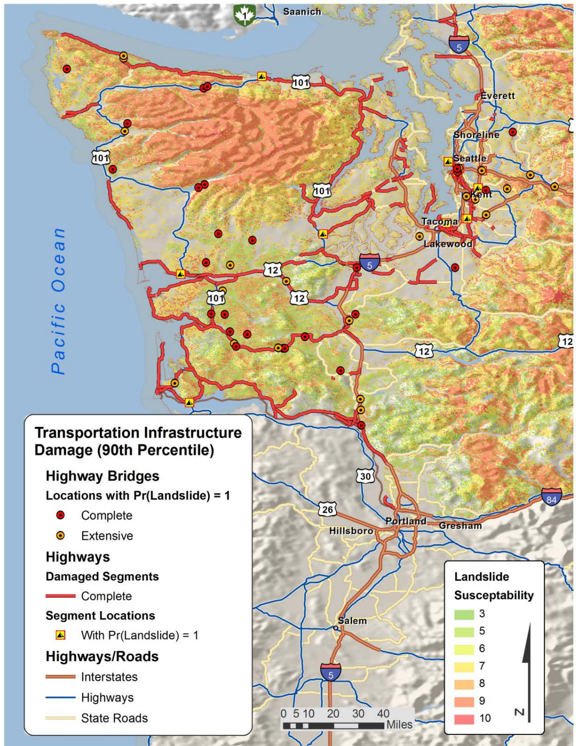
Figure 4-32. Washington transportation infrastructure damage (90th-percentile case)
