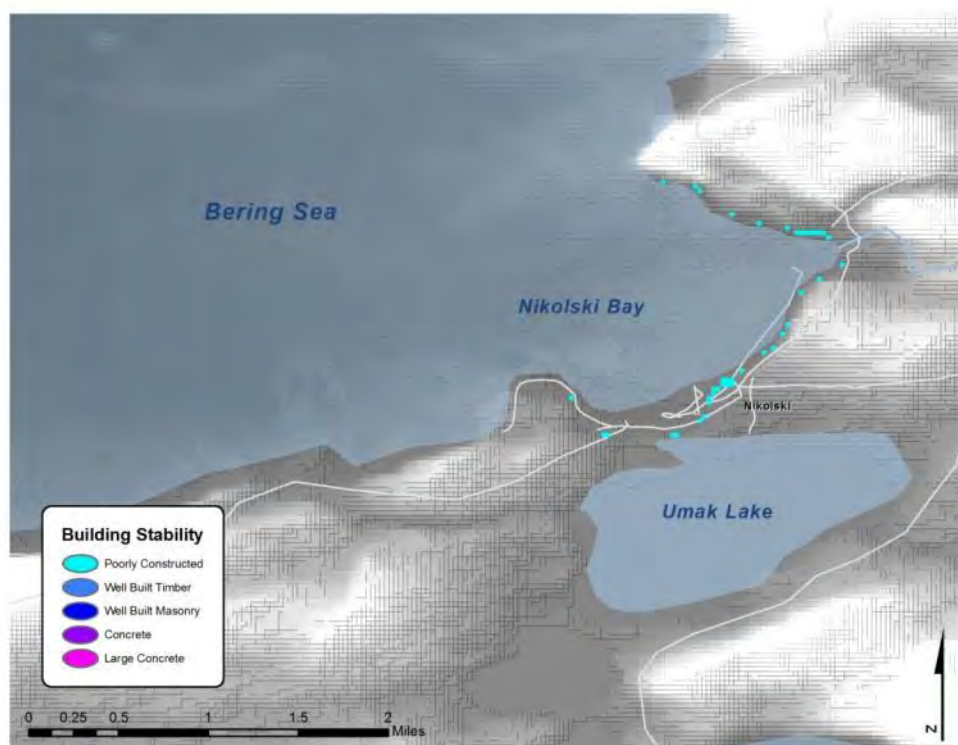
Figure B-7. Predicted building stability rating for Nikolski, AK
