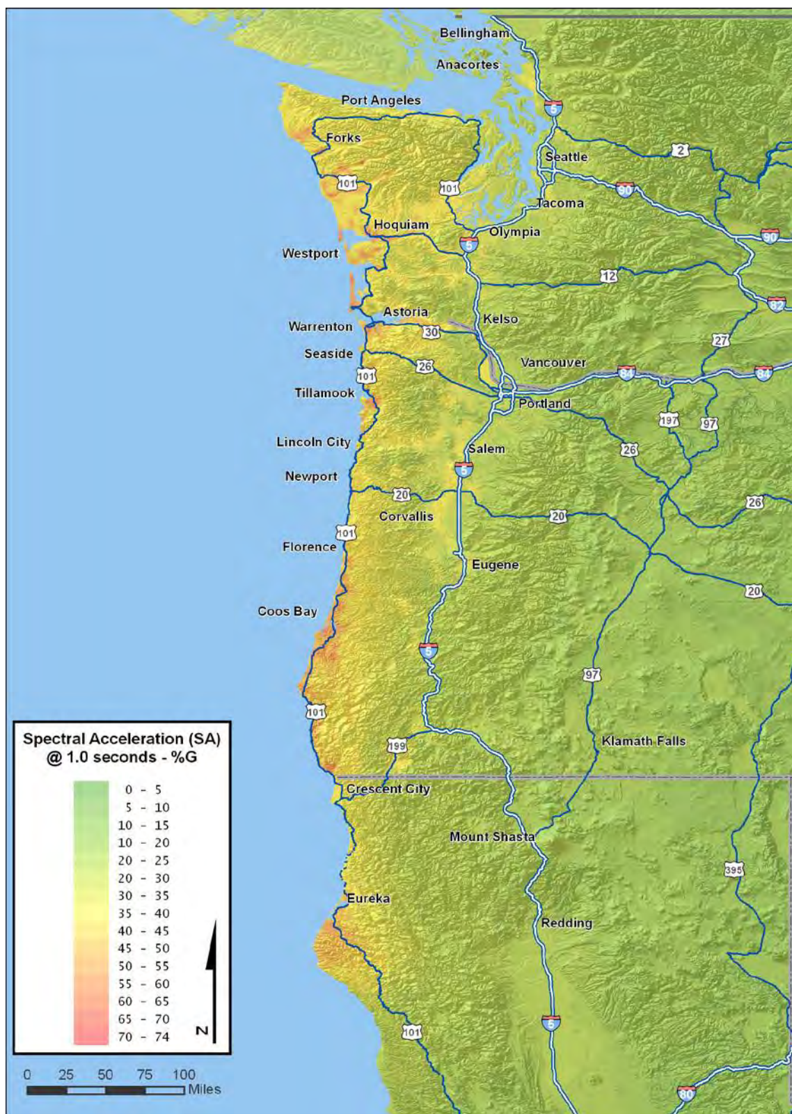
Figure 2-6. Spectral acceleration at 1.0 seconds (percent G)
