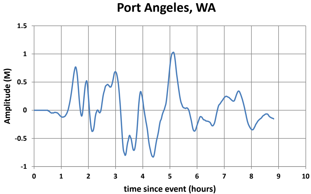
Figure B-70. Port Angeles, WA, Seismic Event Marigram
