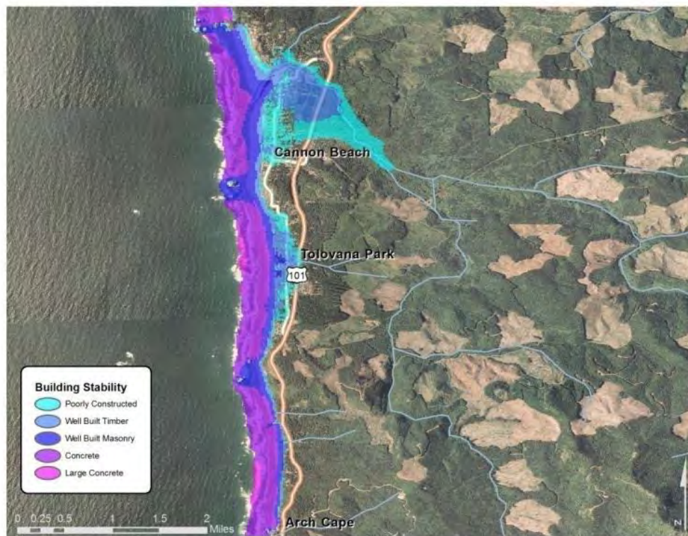
Figure B-29. Predicted building stability rating for Cannon Beach, OR
