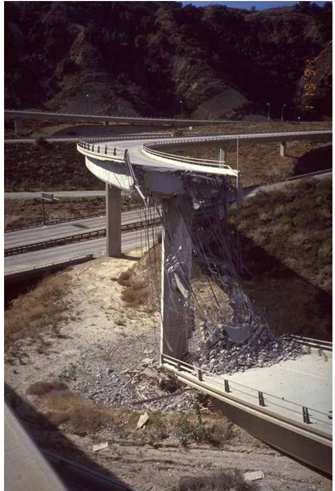
Figure 27. Following the 1994 M6.7 Northridge Earthquake in California, several freeway bridges such as this post-tensioned north to south connector ramp, completely collapsed. Heavily damaged and collapse of bridges that have not been seismically retrofitted may severely disrupt transportation and take years to demolish and rebuild. Photo: Guillermo Santana.
