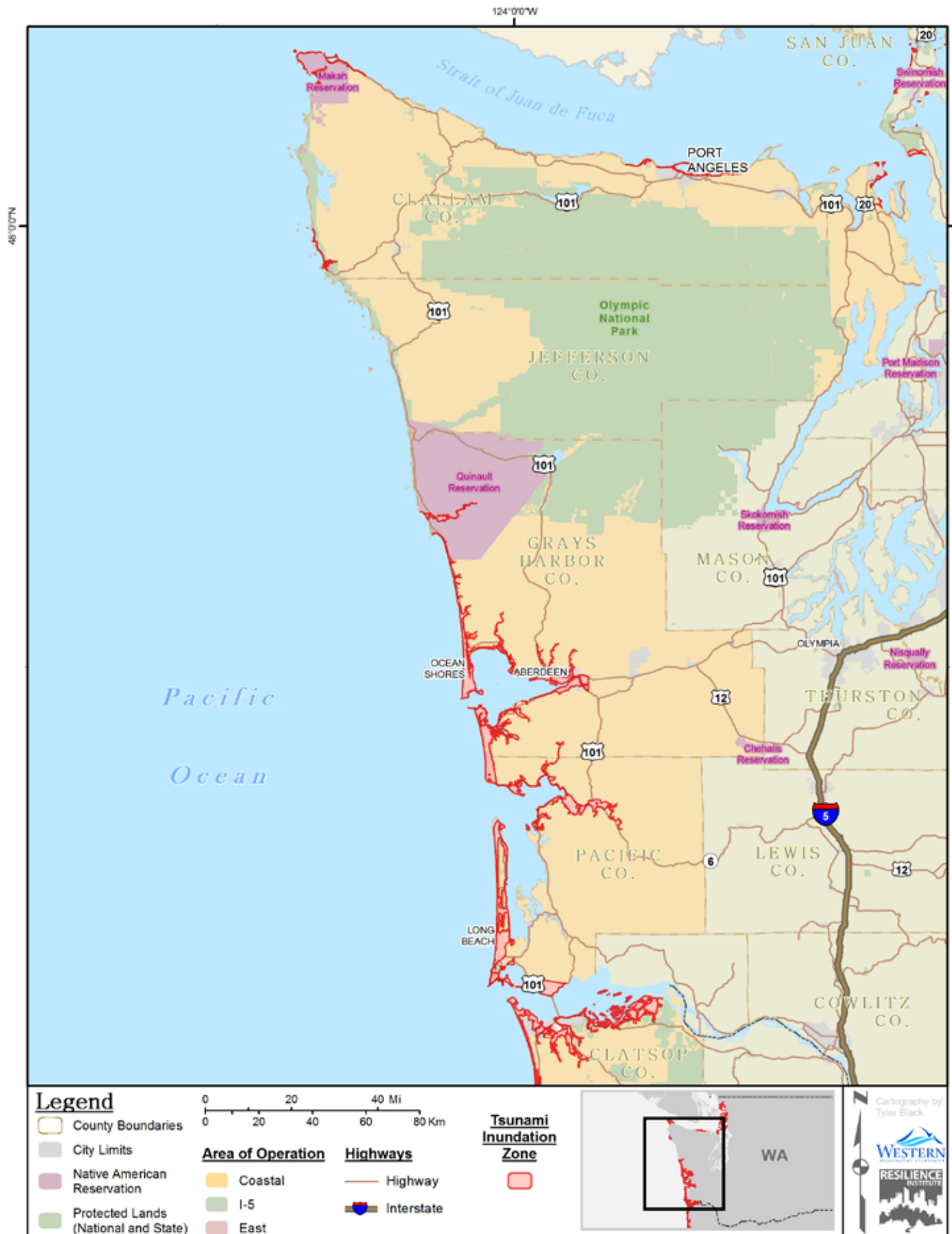
Figure 11. Tsunami inundation zone along the Pacific Coast of Washington
