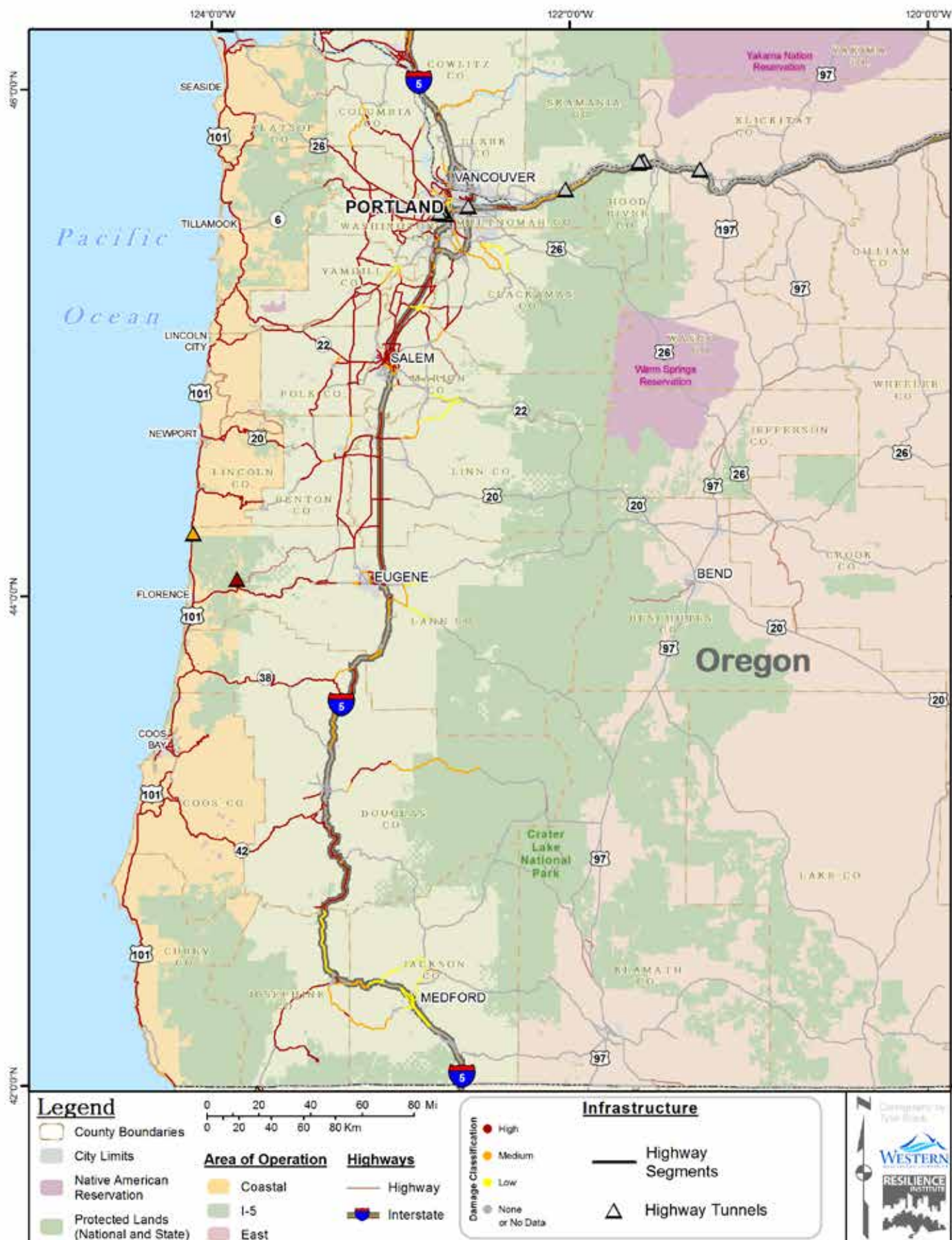
Figure 23. Oregon road and tunnel damage caused by the initial earthquake
