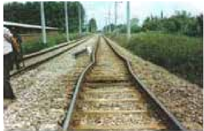
Figure 42. The M 7.4 earthquake in Turkey caused localized bending of the rail tracks. Photo: Turkish State Railways.
