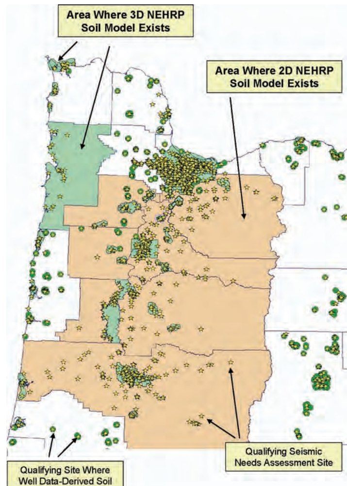
Figure 17. Relationship of areas of NEHRP soil models to seismic assessment sites and ODWR well data based soil profiles.
