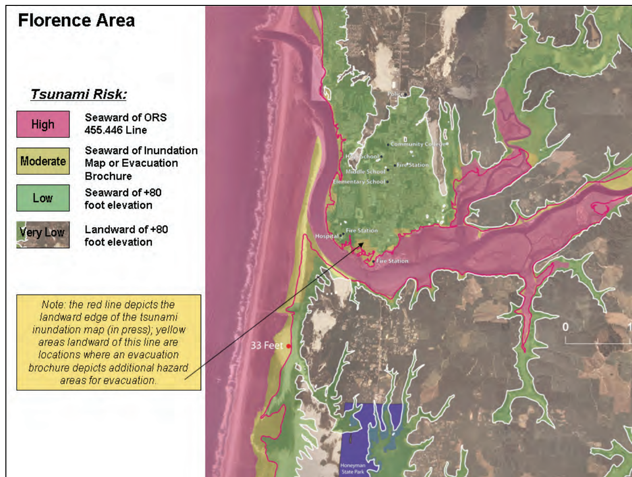
Figure 34. Computer-generated tsunami inundation zones for Florence, Oregon (DOGAMI).
