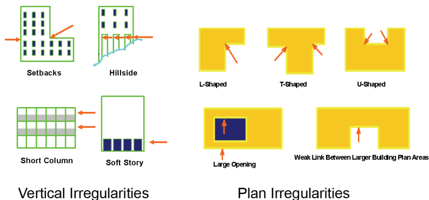
Figure 18. Vertical and plan irregularities describe the shapes of buildings and impact building performance during an earthquake. See Appendix J.
