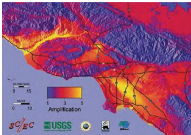
Figure 5. Earthquake ground motion amplification in southern California. Shaking was much greater on landfill or soft soil (USGS).
