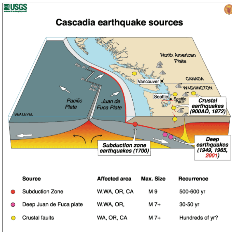
Figure 1. Types of earthquakes that affect Oregon (U.S. Geological Survey).
