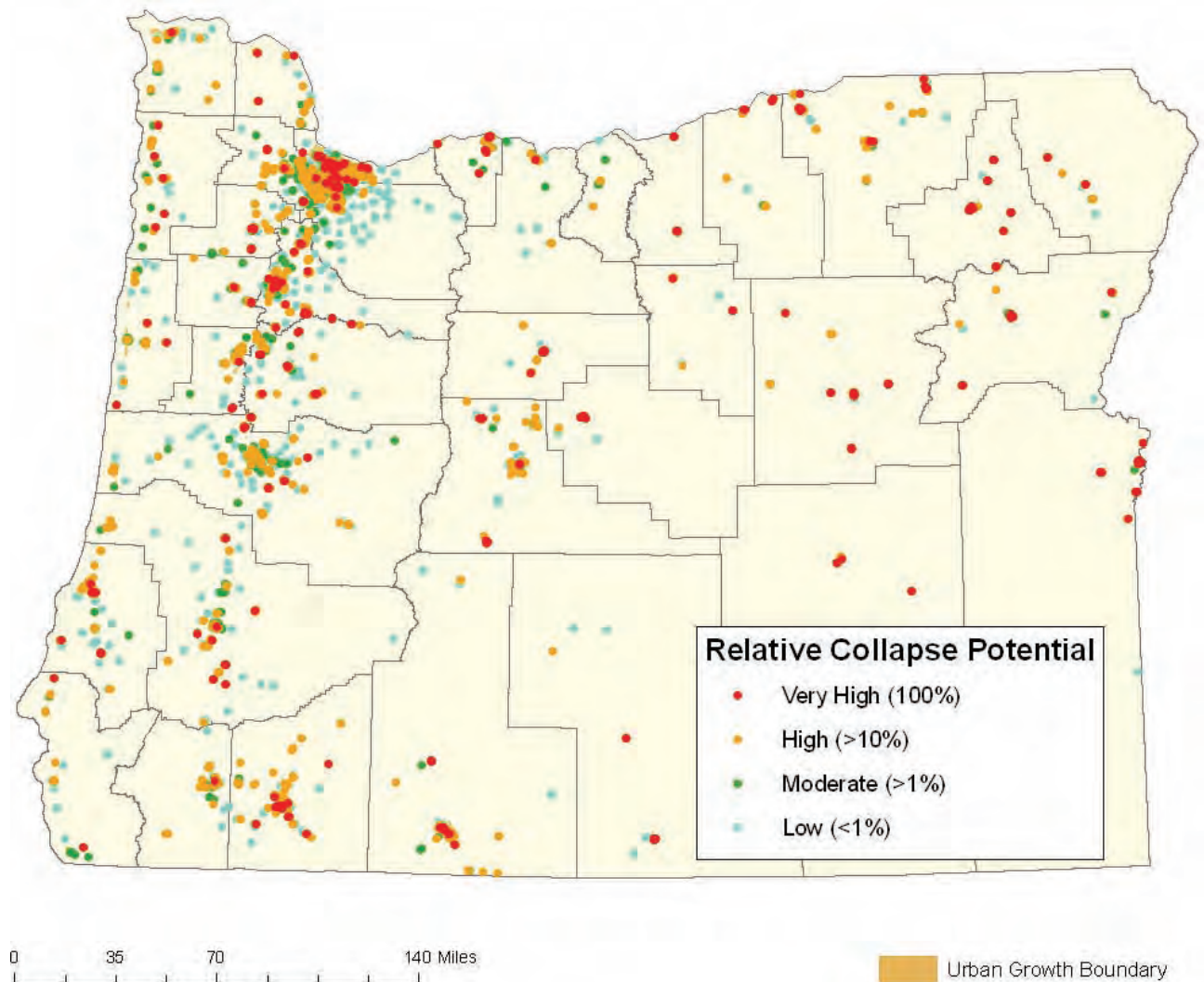
Figure 27. Relative collapse potential for all sites in this seismic needs assessment study.
