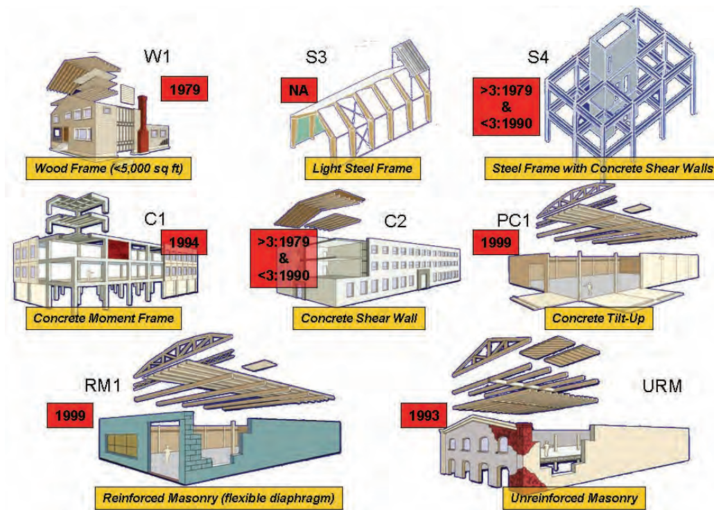
Figure 20. FEMA 154 benchmark dates and building structural types. See Table 7 for definitions. The number 3 in the red boxes indicates greater than or less than 3 stories.
