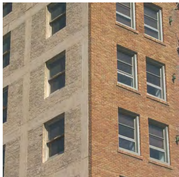
Figure 5-10 Close-up view of 3711 Roxbury Street building exterior showing infill frame construction.
