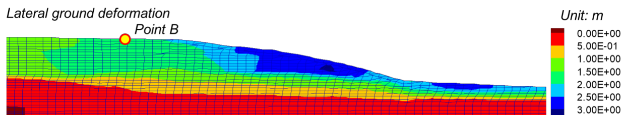
Figure 5-1e: Contours of lateral ground deformation at the end of ground motion #5 in Profile B-B' obtained from 2D nonlinear dynamic analysis in FLAC
