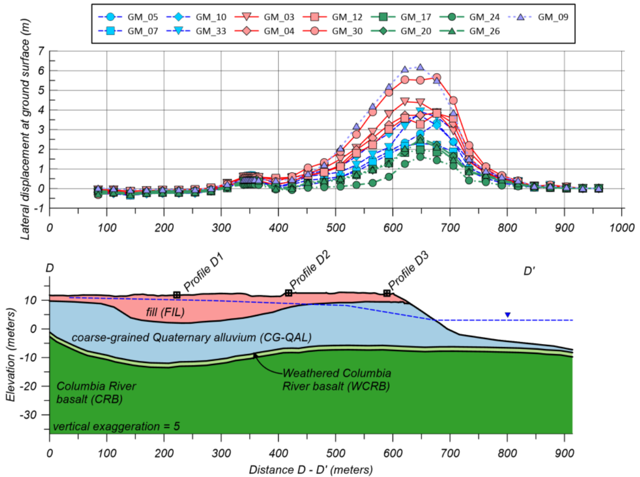
Figure 5-10. Estimates of lateral ground deformations at profile D-D' with coarse-grained QAL based on 2D NDA.
