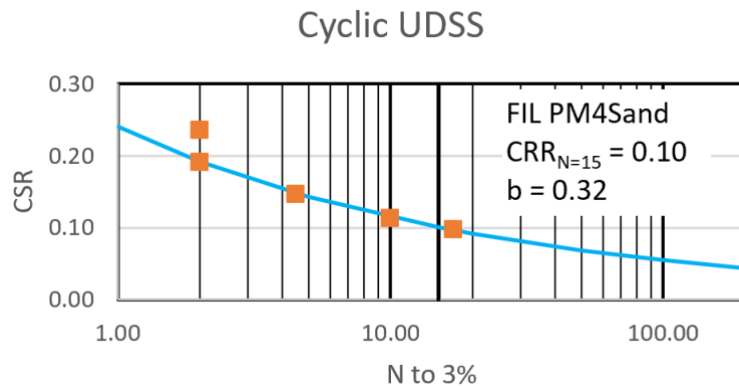
Figure 4-14. Simulated undrained direct simple shear (UDSS) for calibration of FIL for PM4Sand.
