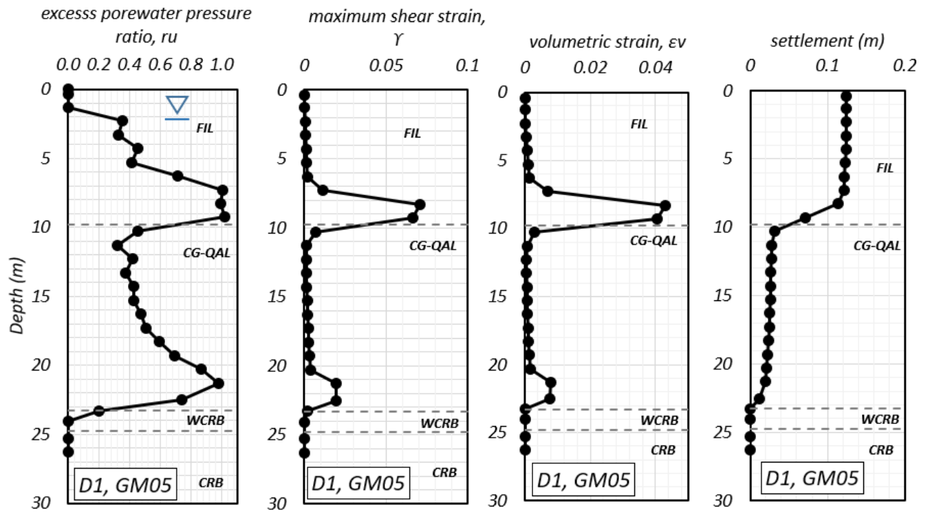
Figure 5-4. Post-liquefaction consolidation settlement estimates at location D1 with coarse-grained QAL and loading from GM05. Settlement estimated with maximum shear strains with Yoshimine et al. (2006).
