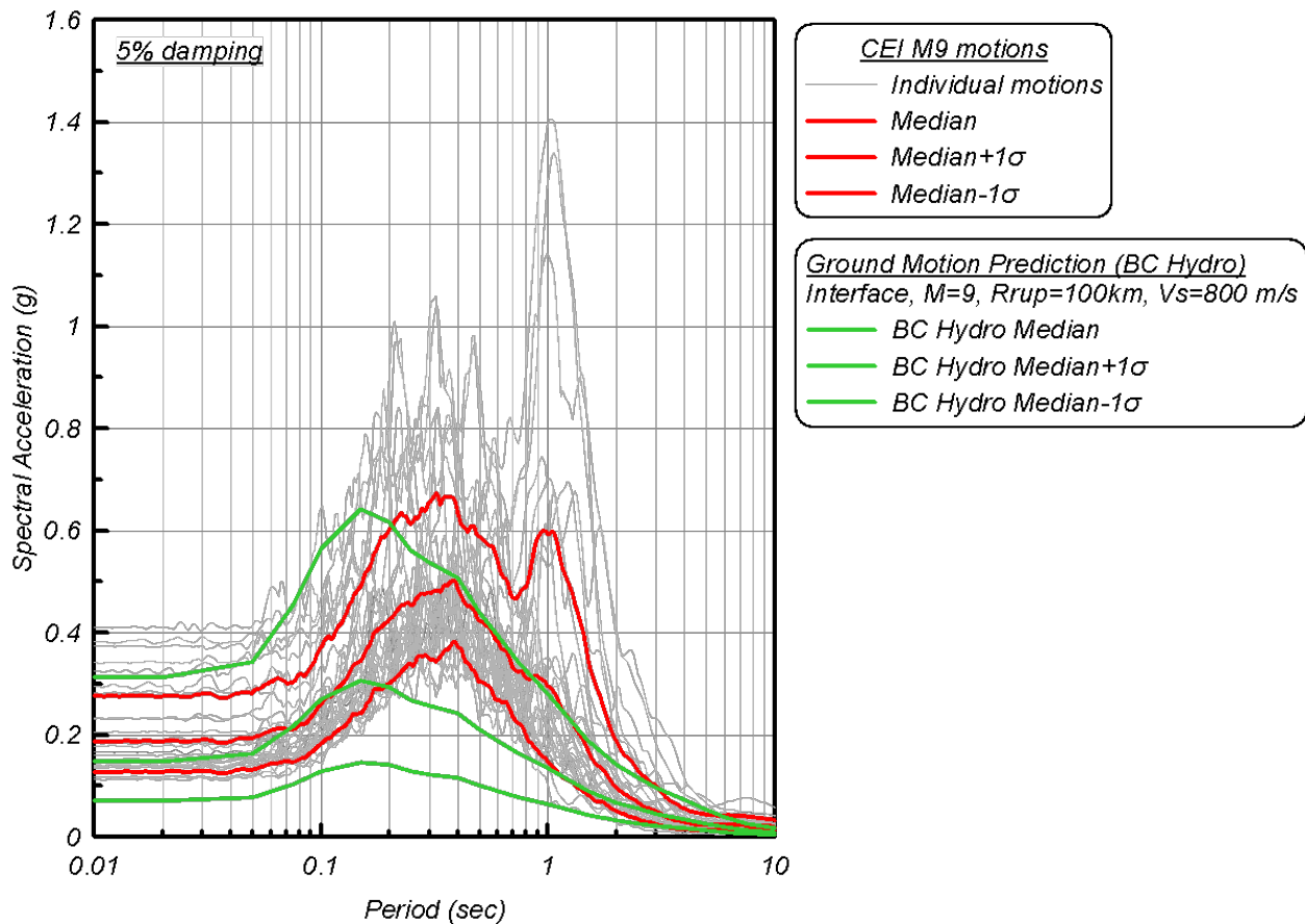
Figure 3-5. Acceleration response spectra of M9 rock ground motions at the CEI hub compared to predictive ground motion model BC-Hydro.
