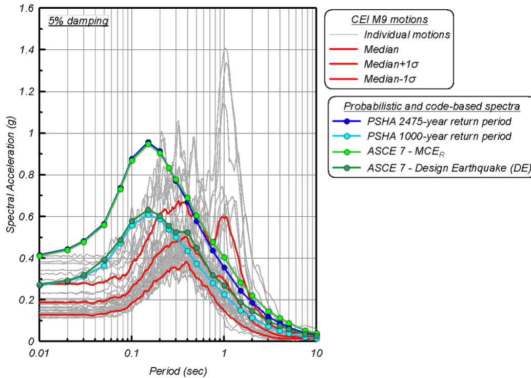
Figure 3-6. Acceleration response spectra of M9 rock ground motions at the CEI hub compared to probabilistic and code-based spectra.
