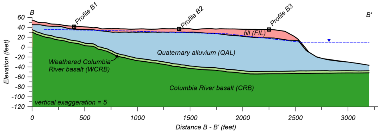
Figure 2-3. Generalized stratigraphy for B-B' profile.
