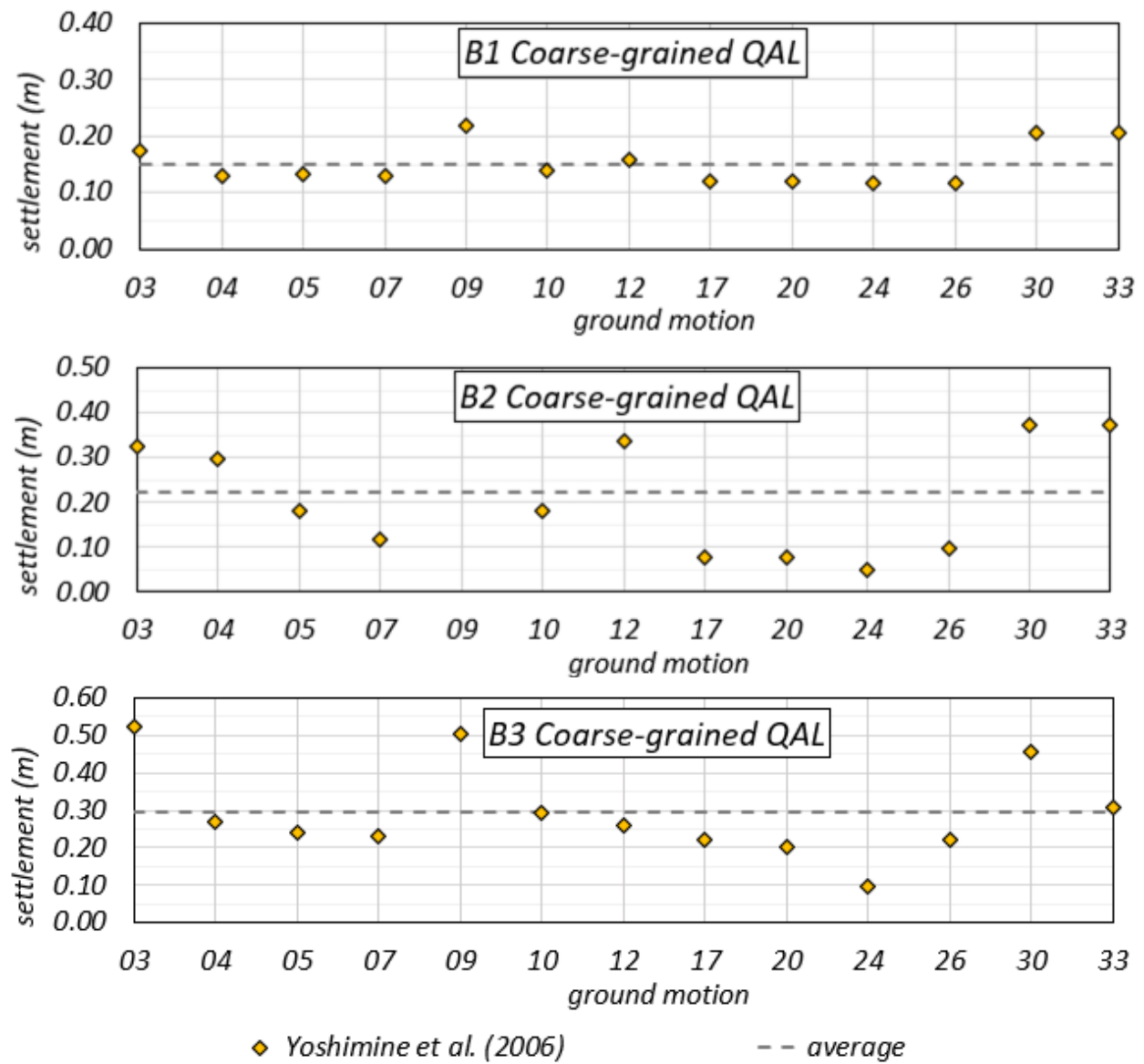
Figure 5-6. Post-liquefaction consolidation settlements estimated at locations B1, B2, and B3 in profile B-B' for CG-QAL. Settlement estimated with maximum shear strain from 2D analysis with Yoshimine et al. (2006) method.
