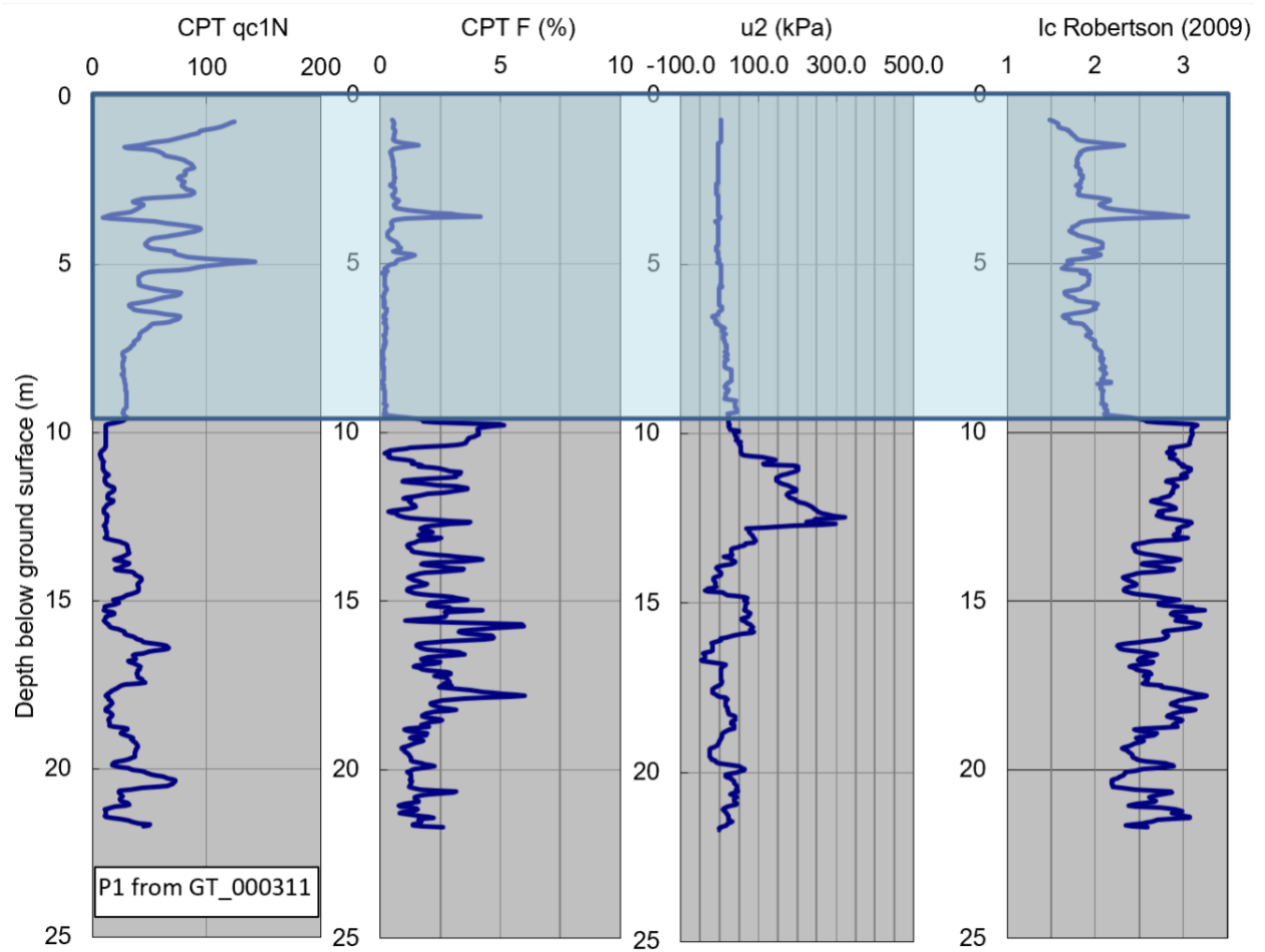
Figure 4-12. CPT data profile P1 located near profile D-D' with presence of FIL. CPT data from report 000311 (GeoEngineers 1995).
