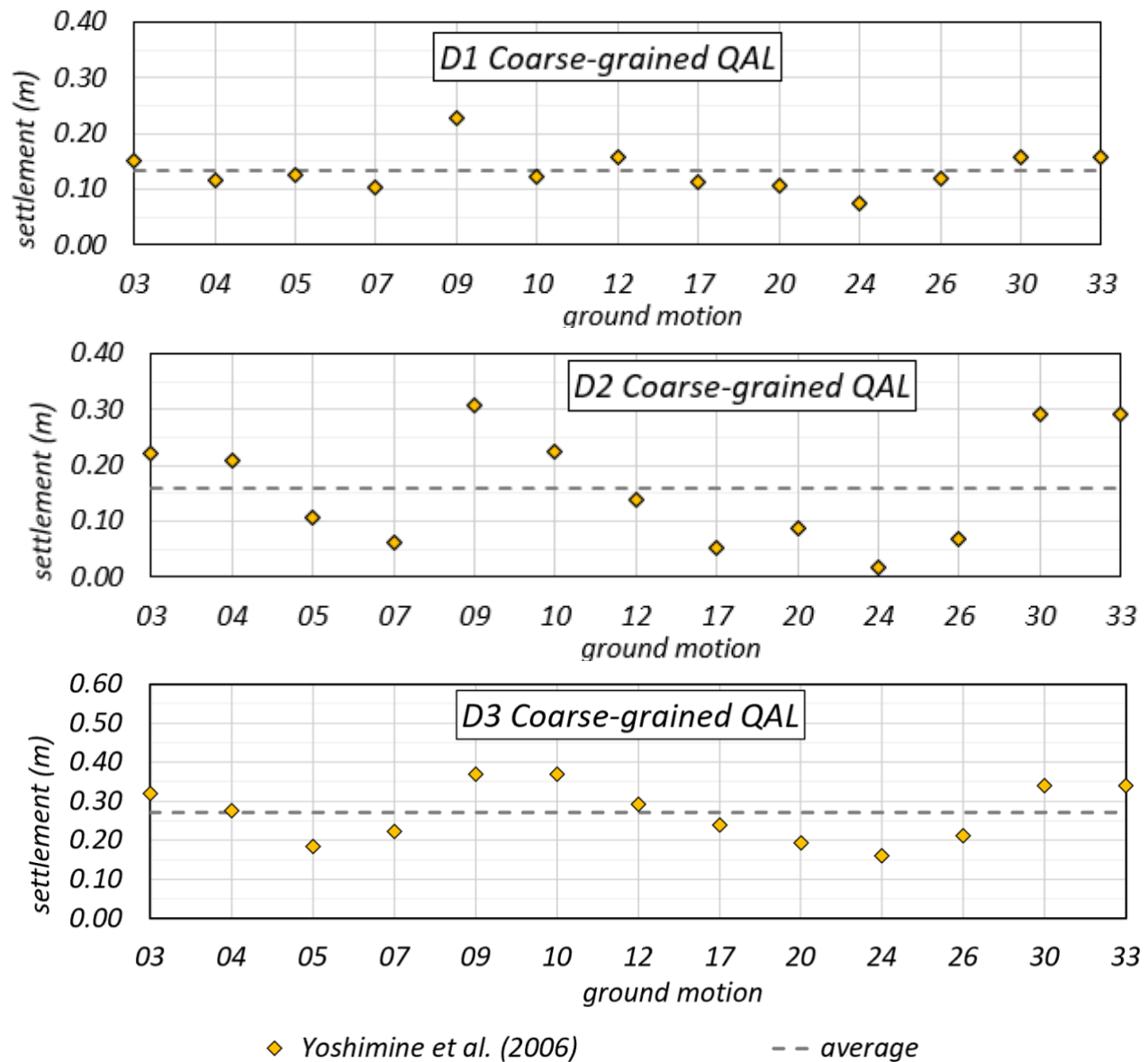
Figure 5-7. Post-liquefaction consolidation settlements estimated at locations D1, D2, and D3 in profile D-D' for CG-QAL. Settlement estimated with maximum shear strain from 2D analysis with Yoshimine et al. (2006) method.
