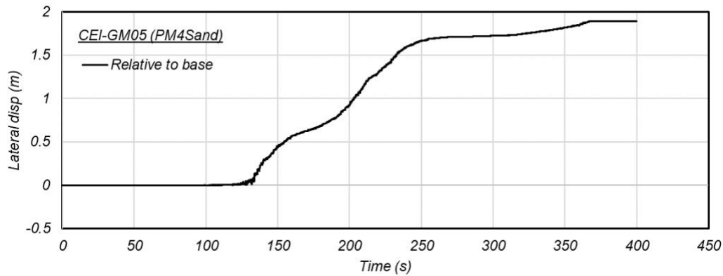
Figure 5-1f: Time history of lateral ground deformation at Point B in Profile B-B' during ground motion #5
