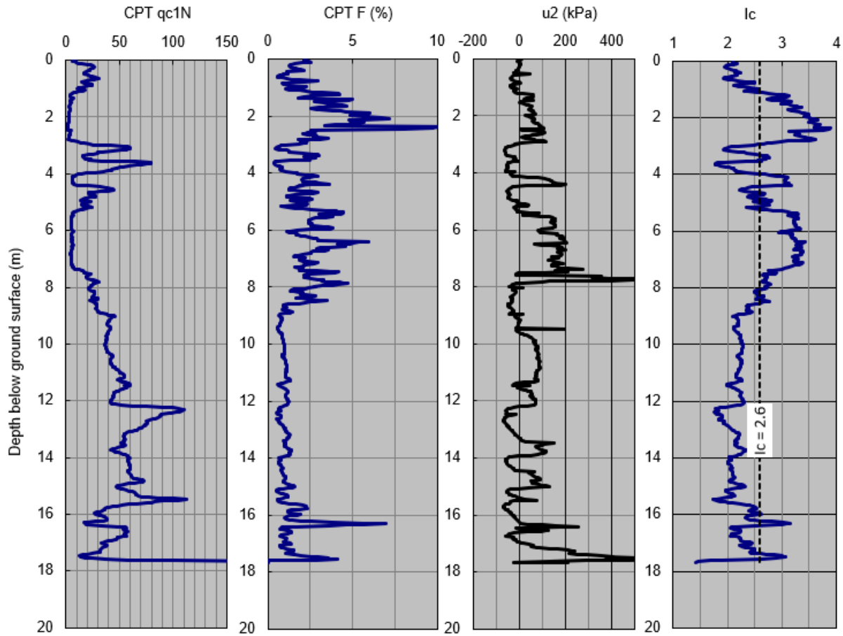
Figure 4-3. CPT-05 profile from PSU's research site north of the CEI hub (Portland General Electric site). Profiles show two types of QAL soils: clay-like QAL with I_c > 2.6 and sand-like QAL with I_c < 2.6 .
