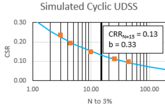
Figure 4-10. Simulated results from cyclic UDSS with the selected PM4Sand parameters for CG-QAL.
