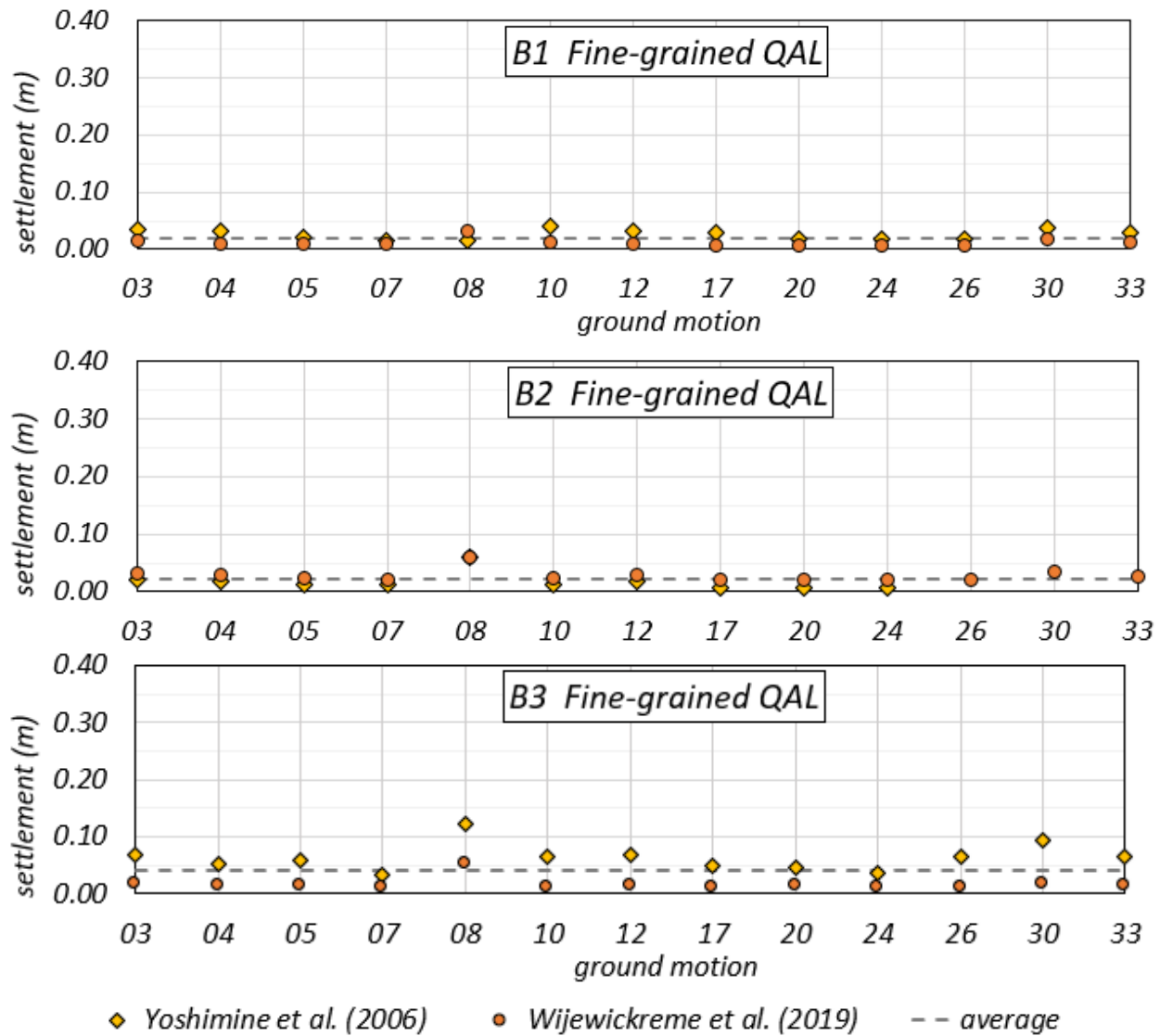
Figure 5-5. Post-liquefaction consolidation settlements estimated at locations B1, B2, and B3 in profile B-B' for FG-QAL. Settlement estimated with maximum shear strain from 2D analysis with Yoshimine et al. (2006) and final excess pore pressure ratio with Wijewickreme et al. (2019) methods.
