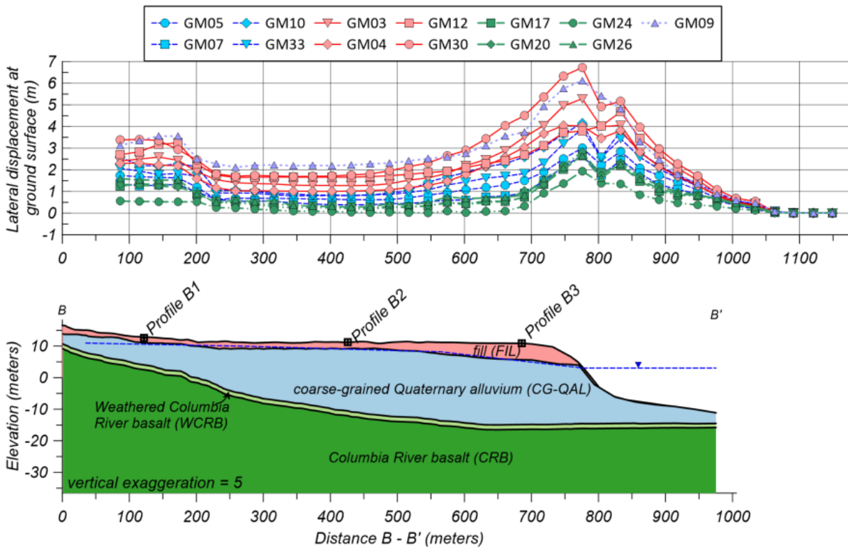
Figure 5-8. Simulated lateral deformations for profile B-B' with coarse-grained QAL.
