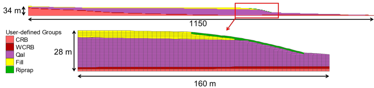
Figure 4-1. Cross section of Profile B-B' in FLAC.
