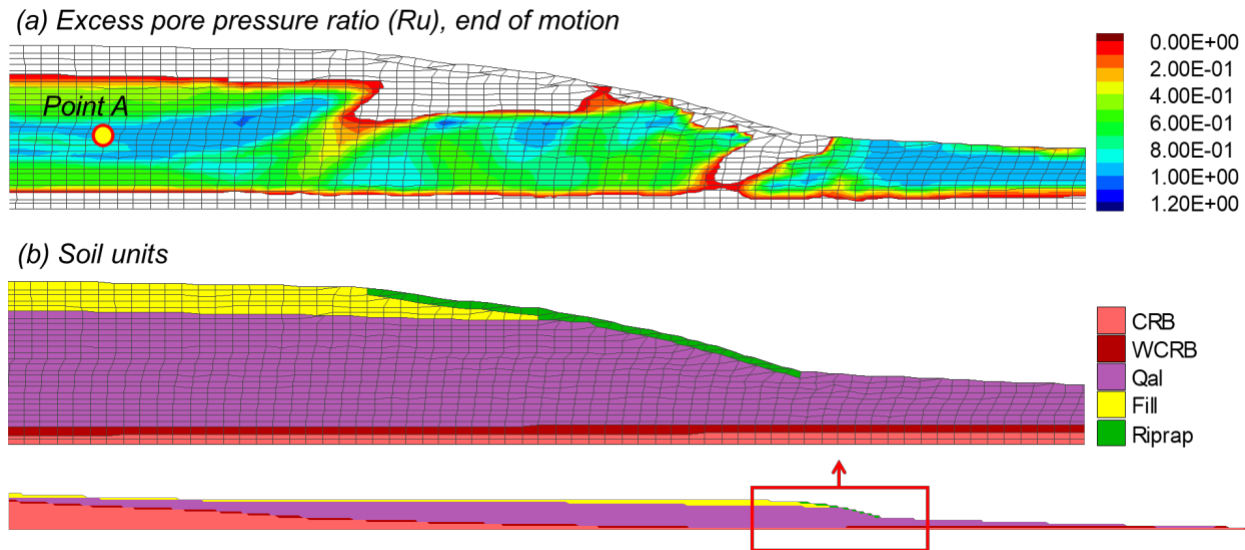
Figure 5-1a: (a) Contours of excess pore pressure ratios at the end of ground motion #5 in Profile B-B' obtained from 2D nonlinear dynamic analysis in FLAC, and (b) soil units
