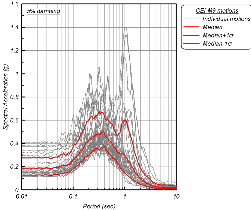
Figure 3-4. Acceleration response spectra of M9 rock ground motions at the CEI hub
