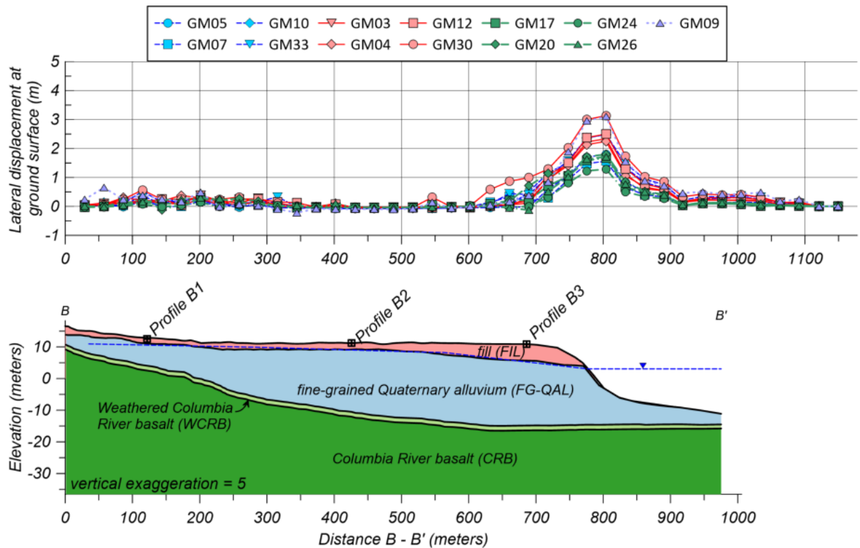
Figure 5-9. Simulated lateral deformations for profile B-B' with fine-grained QAL.
