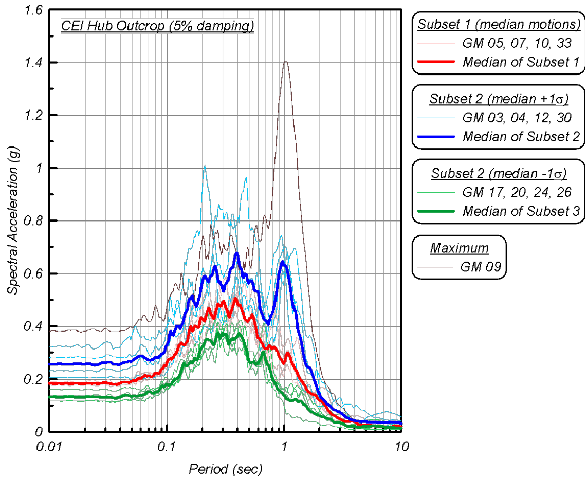
Figure 3-7. Acceleration response spectra for four subsets of CEI M9 rock motions.
