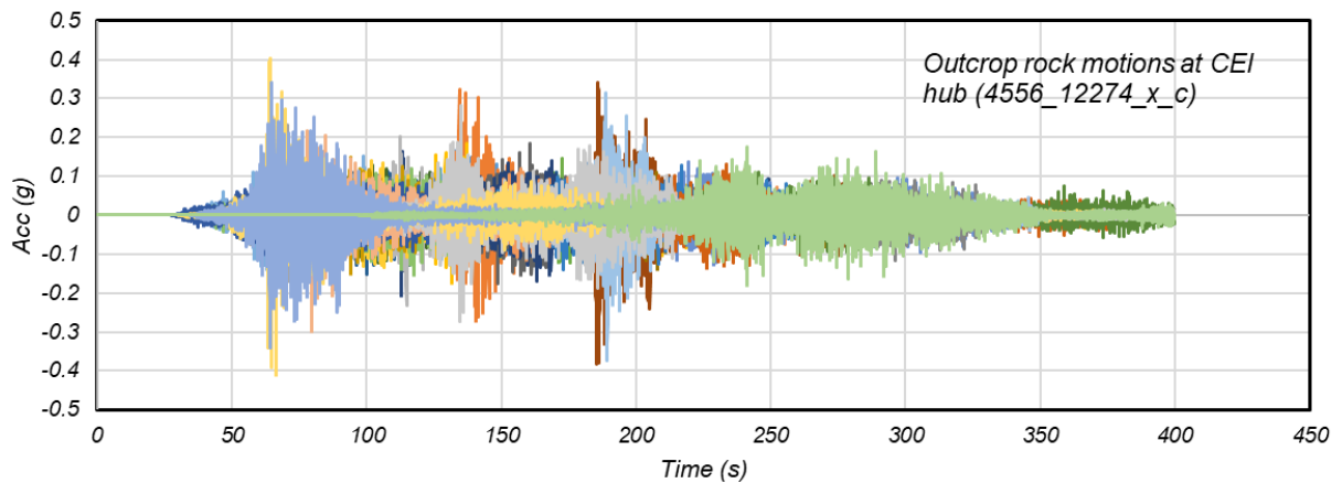
Figure 3-3. Acceleration time histories of M9 rock ground motions at the CEI hub.
