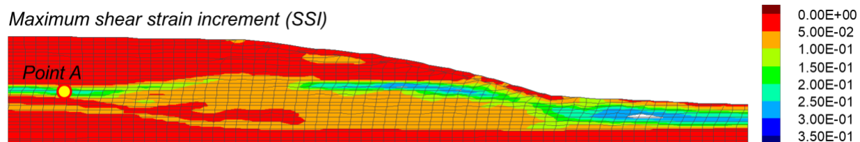
Figure 5-1c: Contours of maximum shear strain increment at the end of ground motion #5 in Profile B-B' obtained from 2D nonlinear dynamic analysis in FLAC
