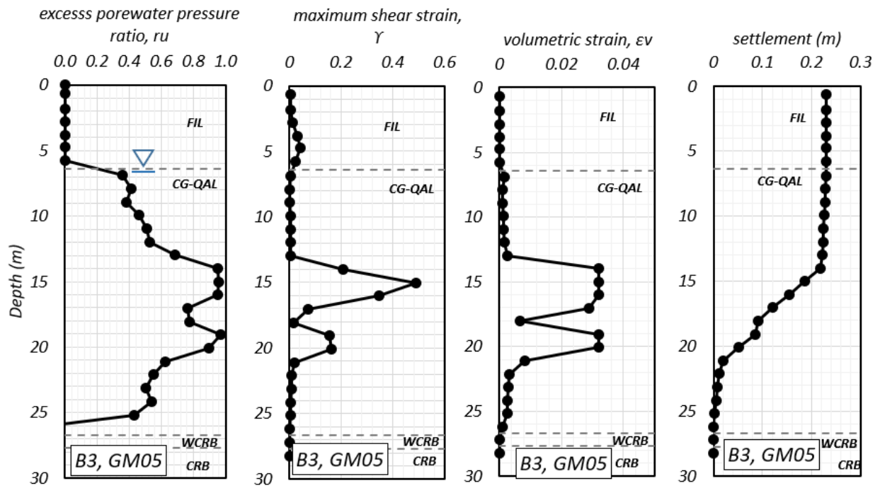
Figure 5-1. Post-liquefaction reconsolidation settlement estimates at location B3 with coarse-grained QAL and loading from GM05.
