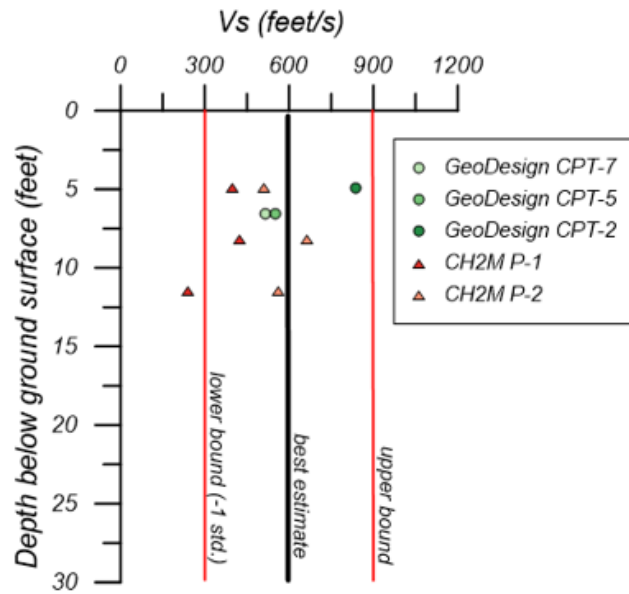
Figure 4-11. Shear wave velocity ( V_s ) measurements from FIL in the CEI hub, including the best estimate of V_s for FIL.
