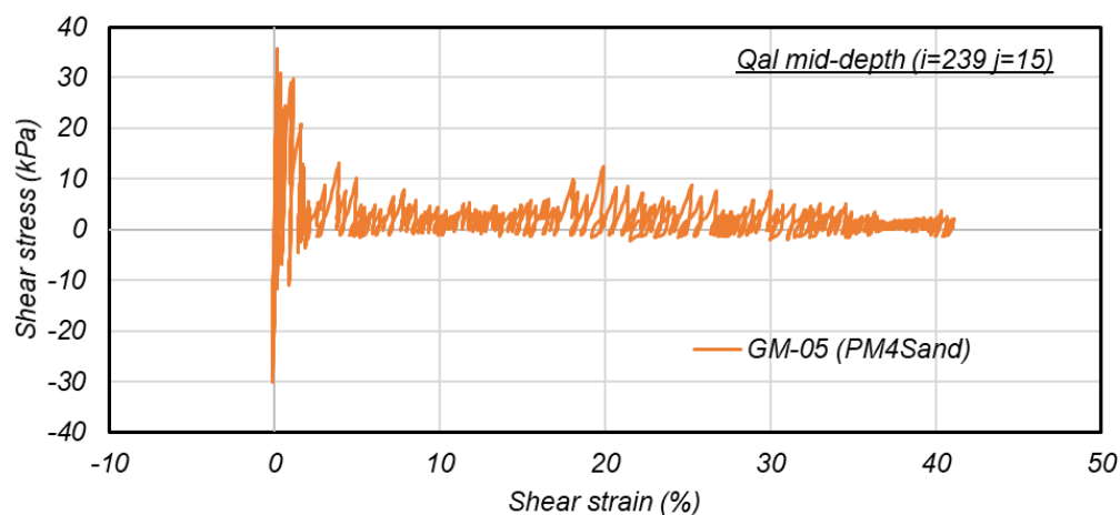
Figure 5-1d: Shear stress versus shear strain for Point A located within the alluvium unit in Profile B-B' during ground motion #5
