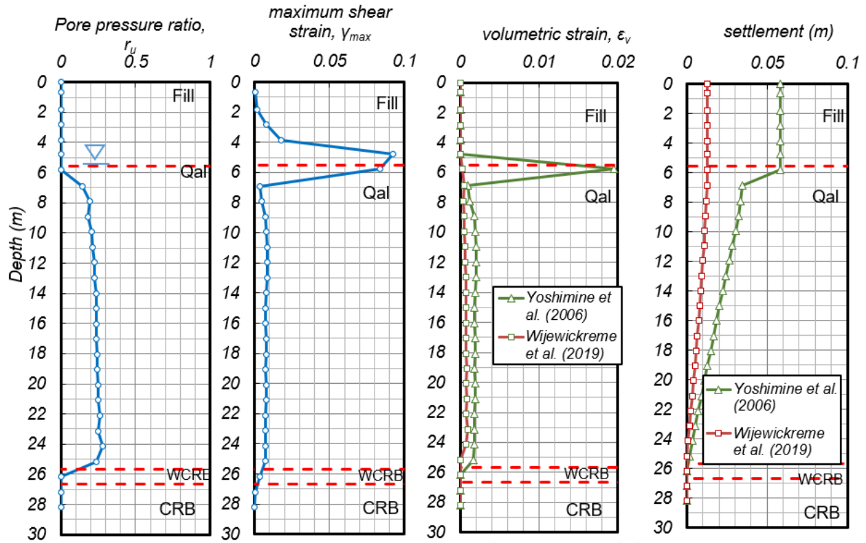
Figure 5-3. Post-liquefaction consolidation settlement estimates at location B3 with fine-grained QAL and loading from GM05. Settlement estimated with maximum shear strains with Yoshimine et al. (2006), and final excess pore pressure ratio with Wijewickreme et al. (2019).
