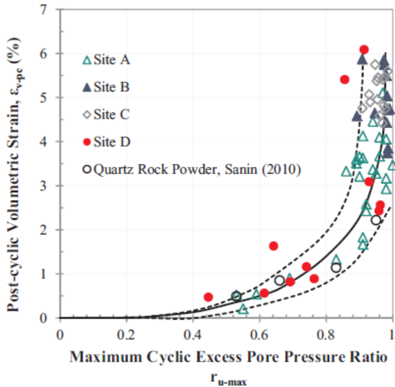
Figure 5-2. Data of post-cyclic volumetric strain vs. excess pore pressure ratio for fine-grained soils (from Wijewickreme et al. 2019).
