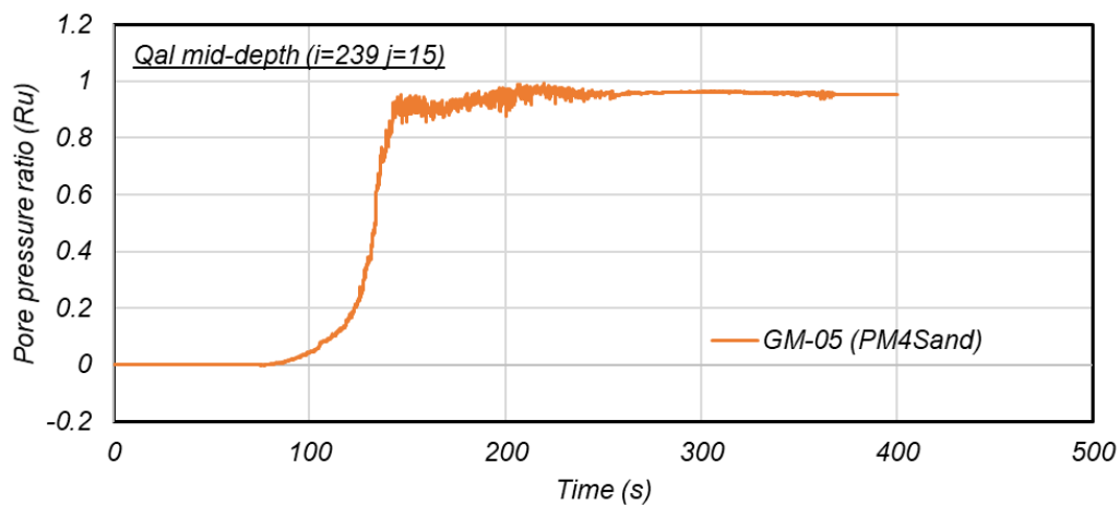
Figure 5-1b: Time history of excess pore pressure ratio for Point A within the alluvium unit in Profile B-B' during ground motion #5
