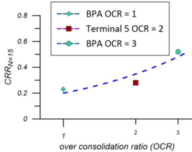
Figure 4-7. Cyclic UDSS testing at OCR = 1, 2, and 3 from O-08 and O-09 sites.
