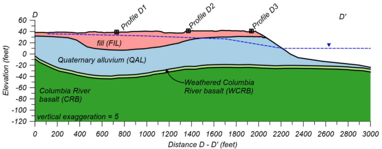
Figure 2-5. Generalized stratigraphy for D-D' profile.
