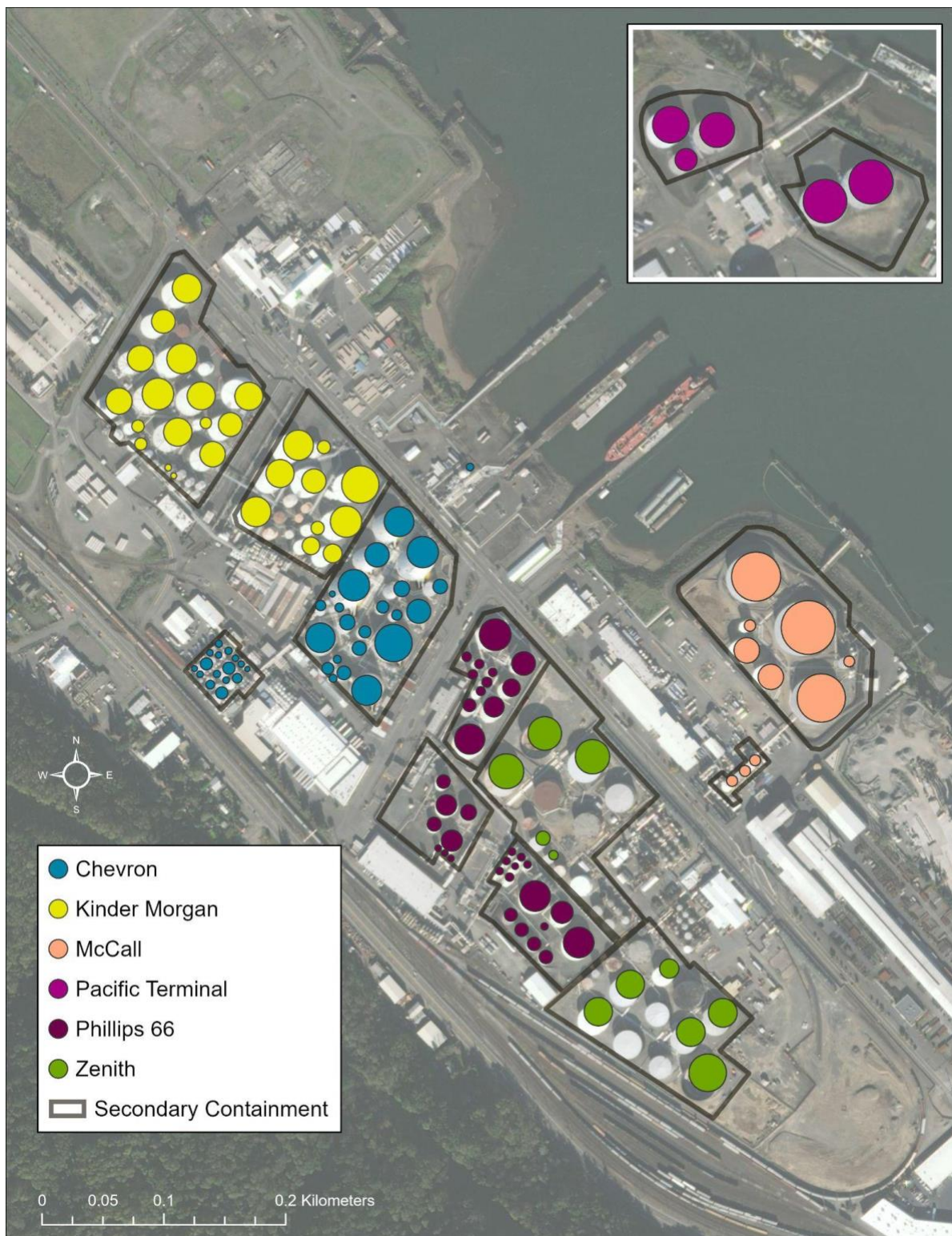
Figure 8-1. Overview of the main CEI Hub located at Willbridge Terminal.
