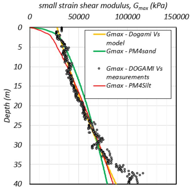
Figure 4-4. G_{maz} versus depth for QAL unit, including the PM4Silt and PM4Sand calibrated relationships.
