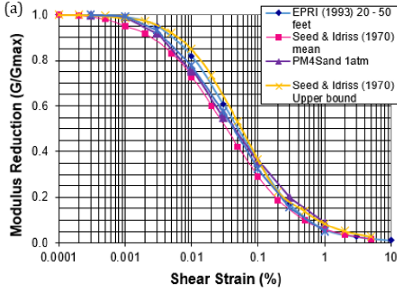
Figure 4-9. Dynamic calibration for CG-QAL with PM4Sand shear modulus reduction relationship.
