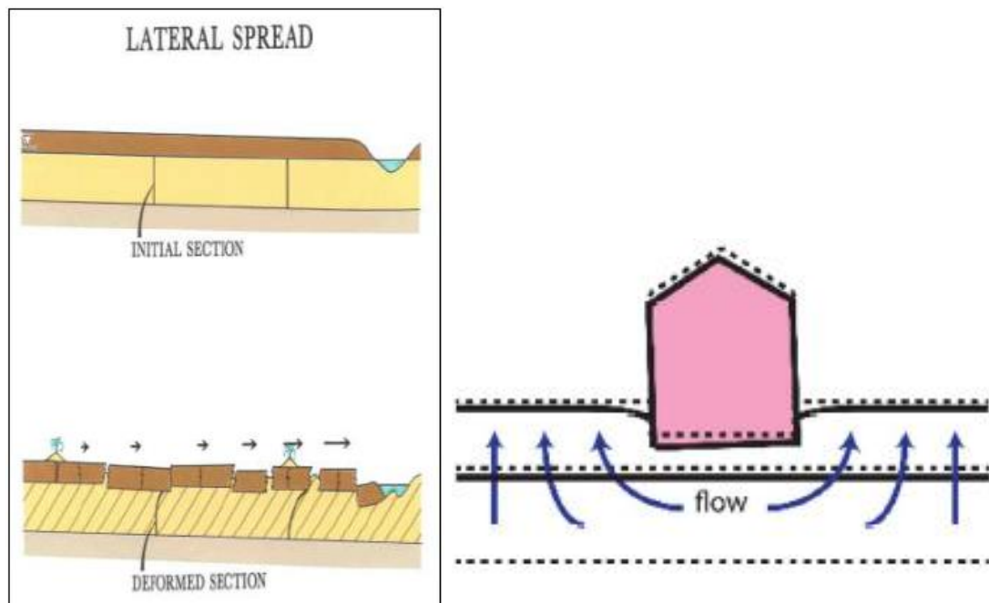
Figure 1-1. Schematic figures showing lateral spreading (from USGS) and settlement due to post-liquefaction settlement (from Bray & Macedo 2017)
