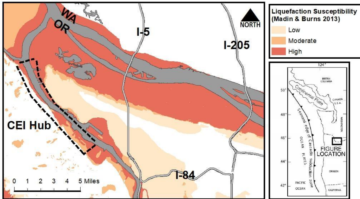
Figure 1-3. Location of the CEI hub and liquefaction susceptibility estimated by Madin & Burns (2013).
