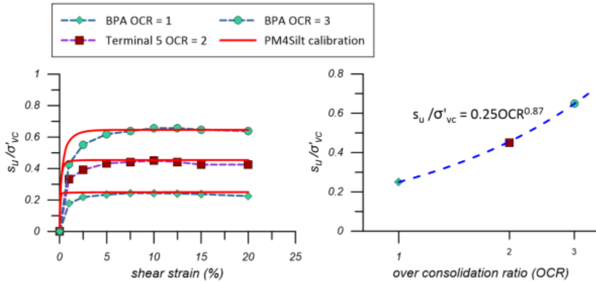
Figure 4-6. Monotonic undrained direct simple shear test results on FG-QAL soils at OCR = 1, 2, and 3.
