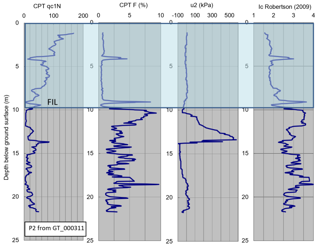
Figure 4-13. CPT data profile P2 located near profile D-D' with presence of FIL. CPT data from report 000311 (GeoEngineers 1995).
