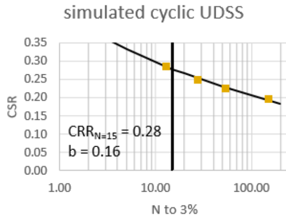
Figure 4-8. Simulated cyclic UDSS testing with PM4Silt to calibrate model parameter h_{po} for FG-QAL behavior.
