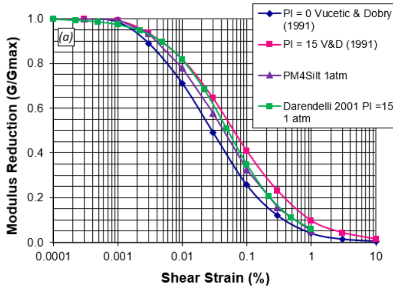
Figure 4-5. Dynamic calibration for FG-QAL with PM4Silt shear modulus reduction relationship.
