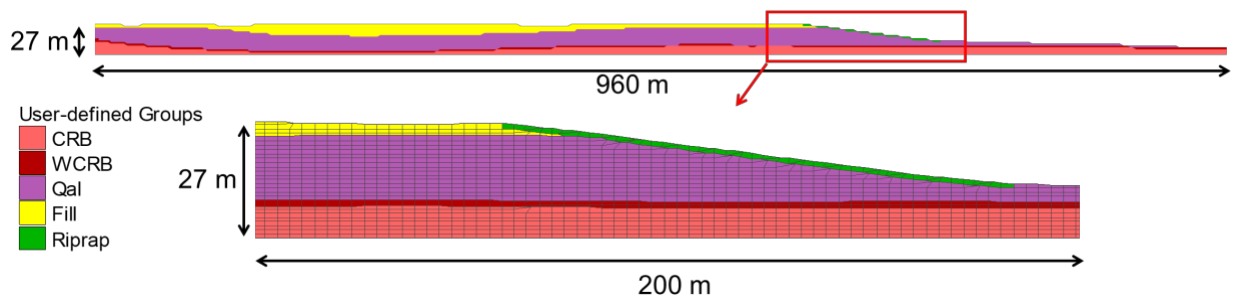
Figure 4-2. Cross section of Profile D-D' in FLAC.
